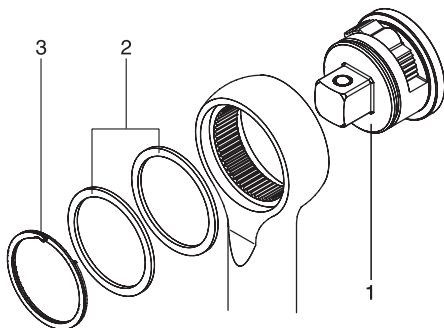
1 Head 2 Ring 3 Retaining Ring
